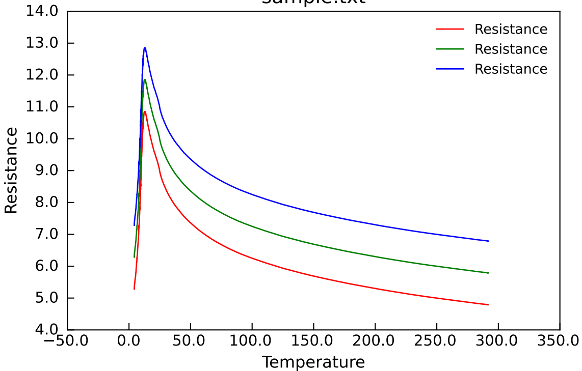
sample.txt
