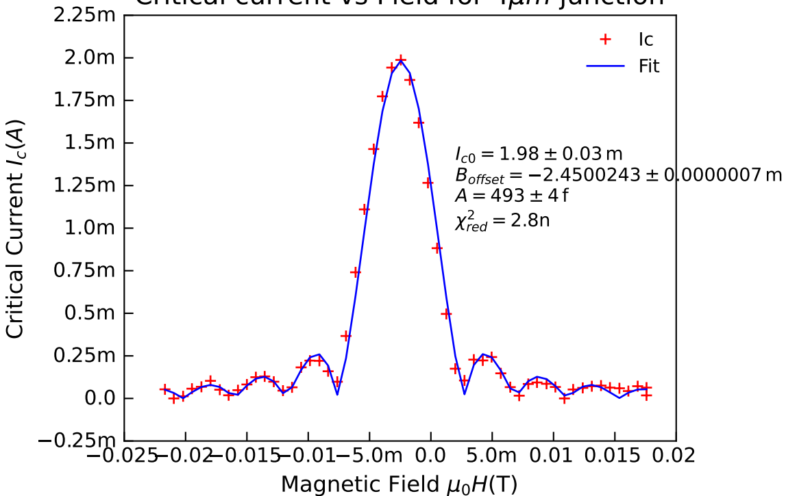
Critical current vs Field for 4\mu\text{m} junction
